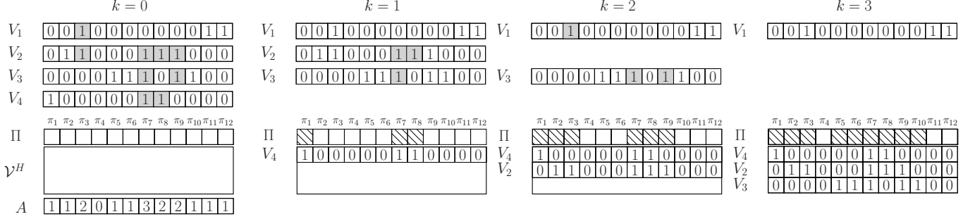
Figure 1: G-SAVMM Execution Example.
